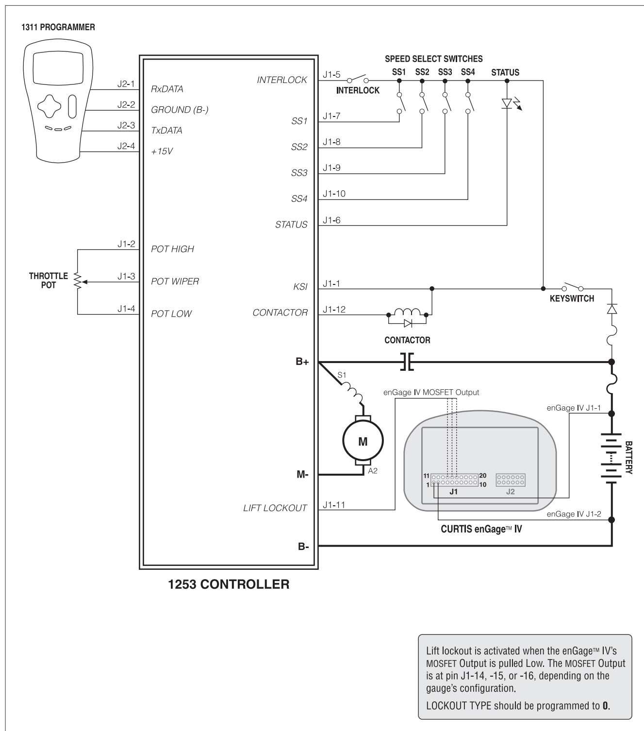
Fig. 3d Standard wiring configuration, Curtis 1253 controller with Curtis enGage™ IV providing lift lockout.
